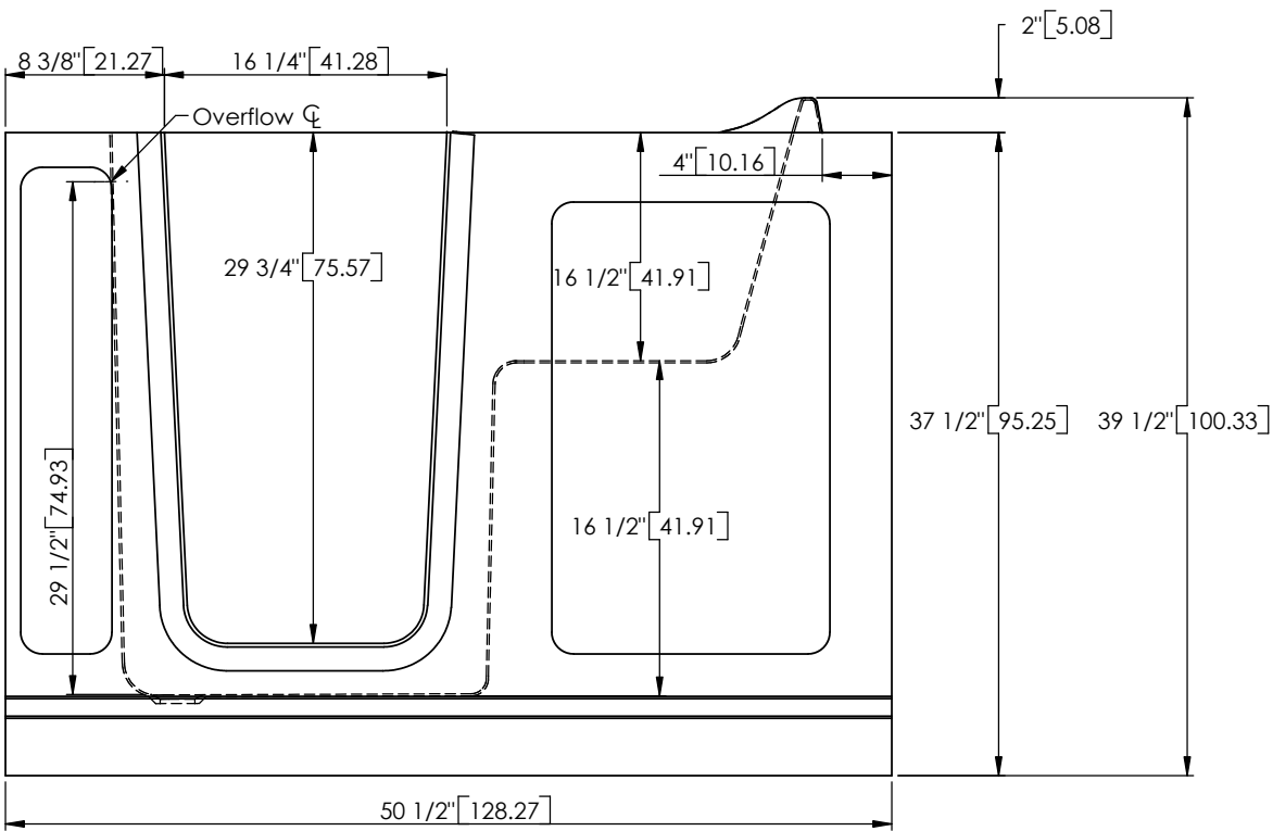
FRONT VIEW
